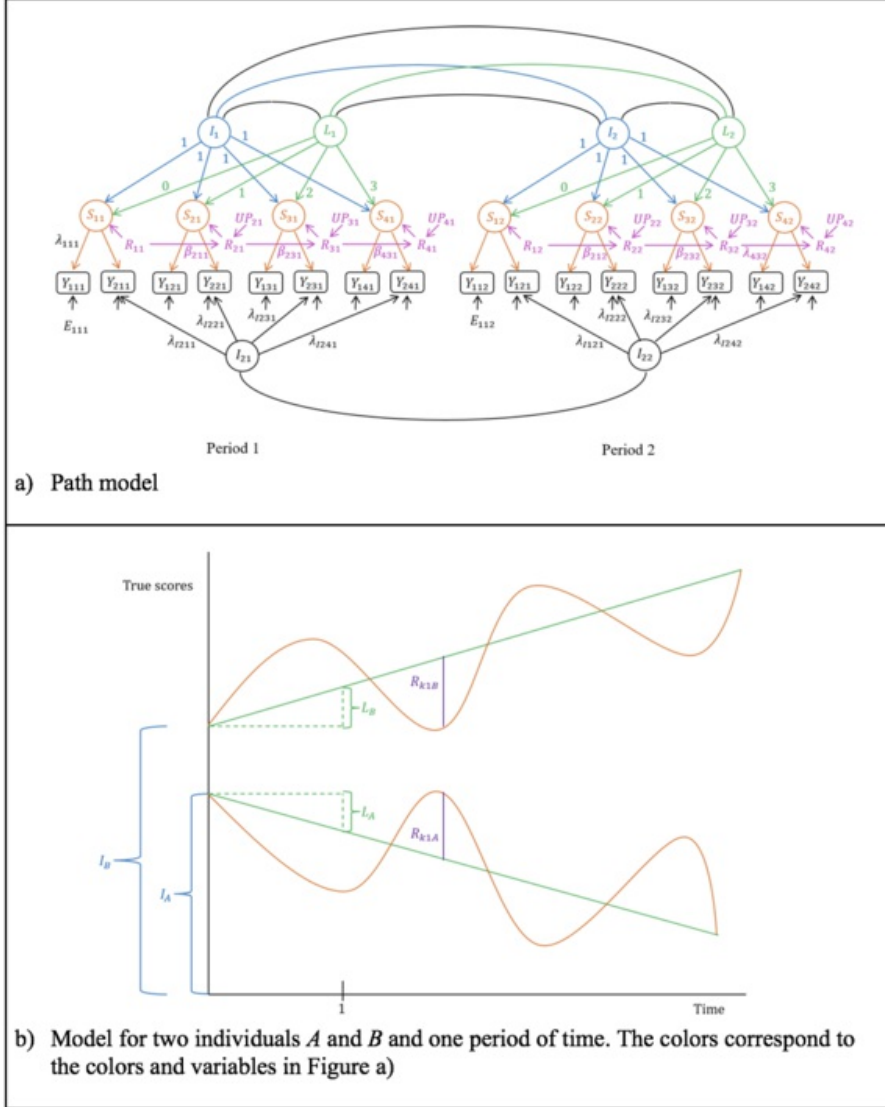
Figure 3. General longitudinal model. Y_{ikp} : observed variables, i : indicator, k : occasion of measurement, p : period. \lambda_{ikp} , \lambda_{Iikp} : loading parameters. E_{ikp} : residual (measurement error variables). I_p : intercept factor, L_p : slope factor, S_{kp} : latent state variable; R_{kp} : occasions-specific residual, U_{kp} : occasion-specific residual indicating unpredictability. \beta_{i(k-1)p} : autoregressive parameter. For reasons of clarity not all parameter labels are included.
